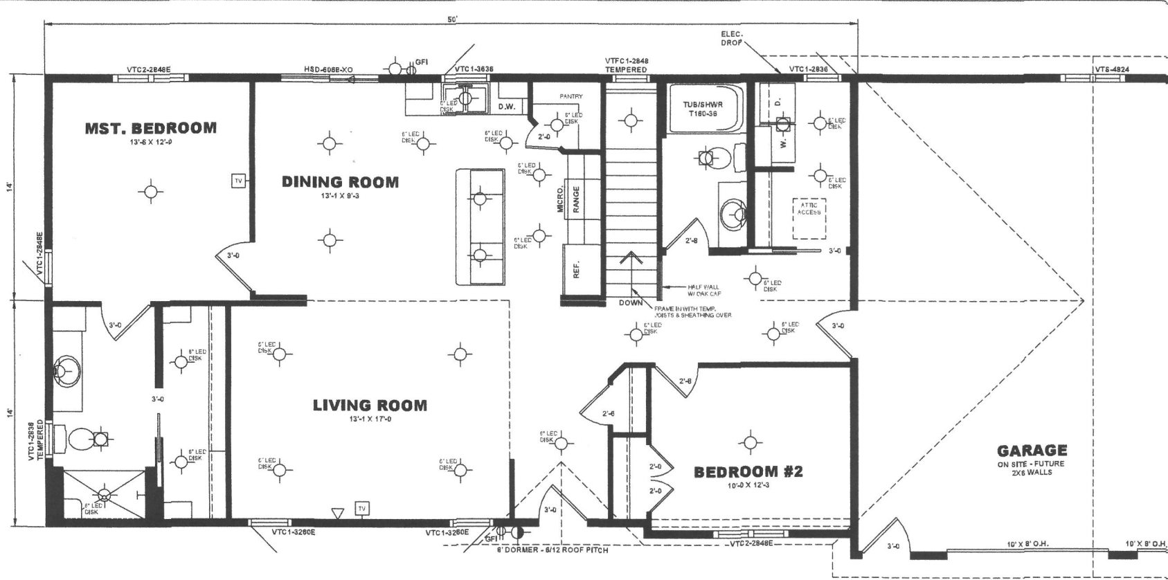
FLOOR PLAN 1/4"=1'-0" (DIMENSIONS FRAMING TO FRAMING)
